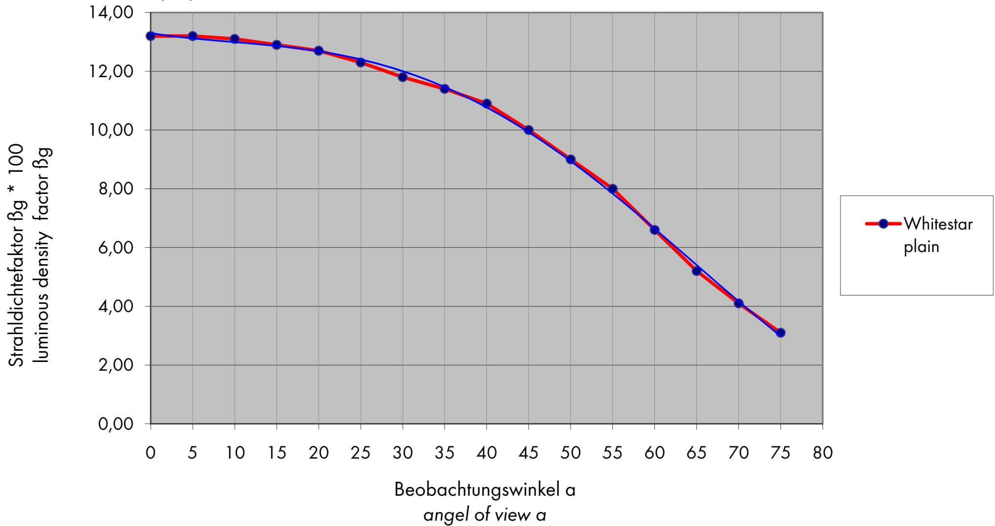
Projektionsfolie WHITESTAR PLAIN - Transmission nach DIN 5036-3 projection screen WHITESTAR PLAIN - transmission acc. to DIN 5036-3
